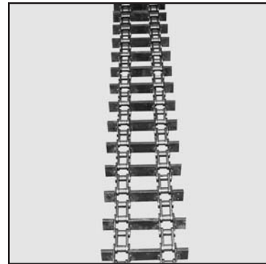
81X Chain 2 Strands with Custom Paddles
