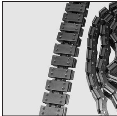
C2082H Lambda Chain with Custom Top Plates and Slider Blocks on Underside
