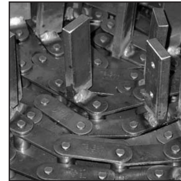
81X Chain Custom Paddle Weld On Attachments
