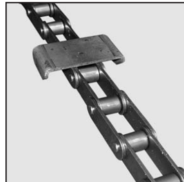
Custom Bent Top Plate for 81X Chain
